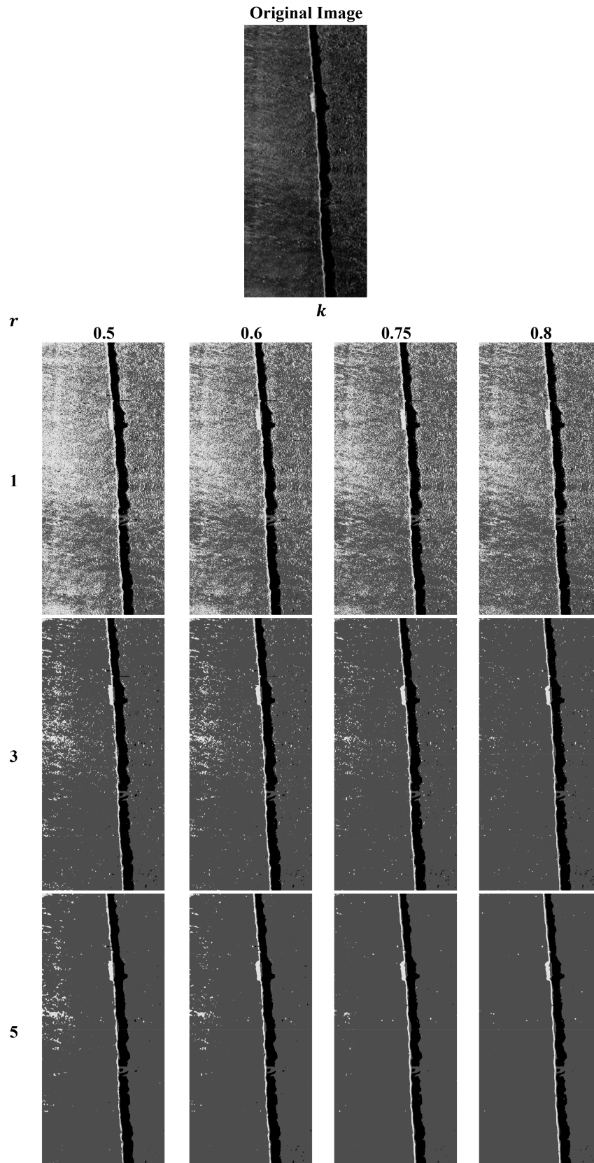
Fig. 7 Sonar image for pipeline detections on the seafloor for different radius sizes r (1, 3 and 5) and order statistics k (0.5, 0.6, 0.75 and 0.8)
