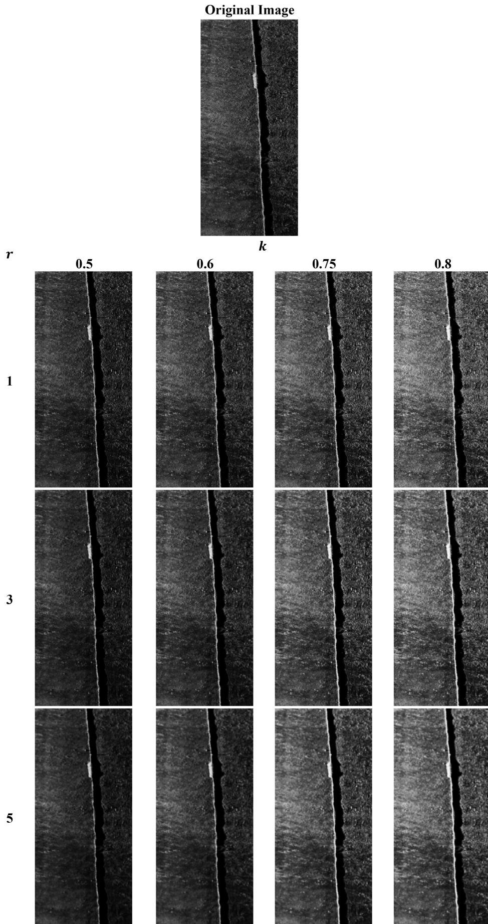
Fig. 5 Visualisation of the k th order statistic value x_k for different radius size r (1, 3 and 5) and order statistics k (0.5, 0.6, 0.75 and 0.8) for sonar image with a pipeline on seafloor
