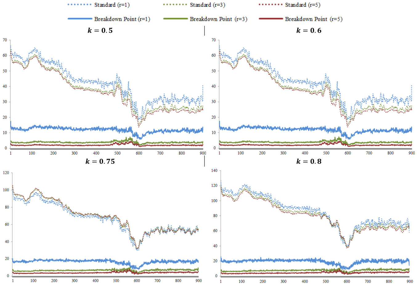
Fig. 6 Column-average bin-displacements for calculation of the k th order statistic value x_k when different r radius sizes (1, 3 and 5) and order statistics k (0.5, 0.6, 0.75 and 0.8) are used
