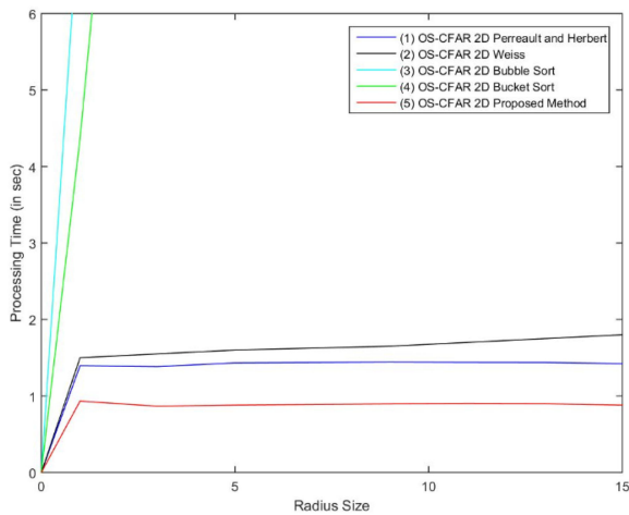
Fig. 10 Processing time versus radius size for OS-CFAR 2D using the (i) Perreault and Herbert method [30] (blue line), (2) Weiss method [28] (black line) (3) bubble sort method [25] (cyan line) (4) bucket sort method [25] (green line) and (5) proposed method (red line)
