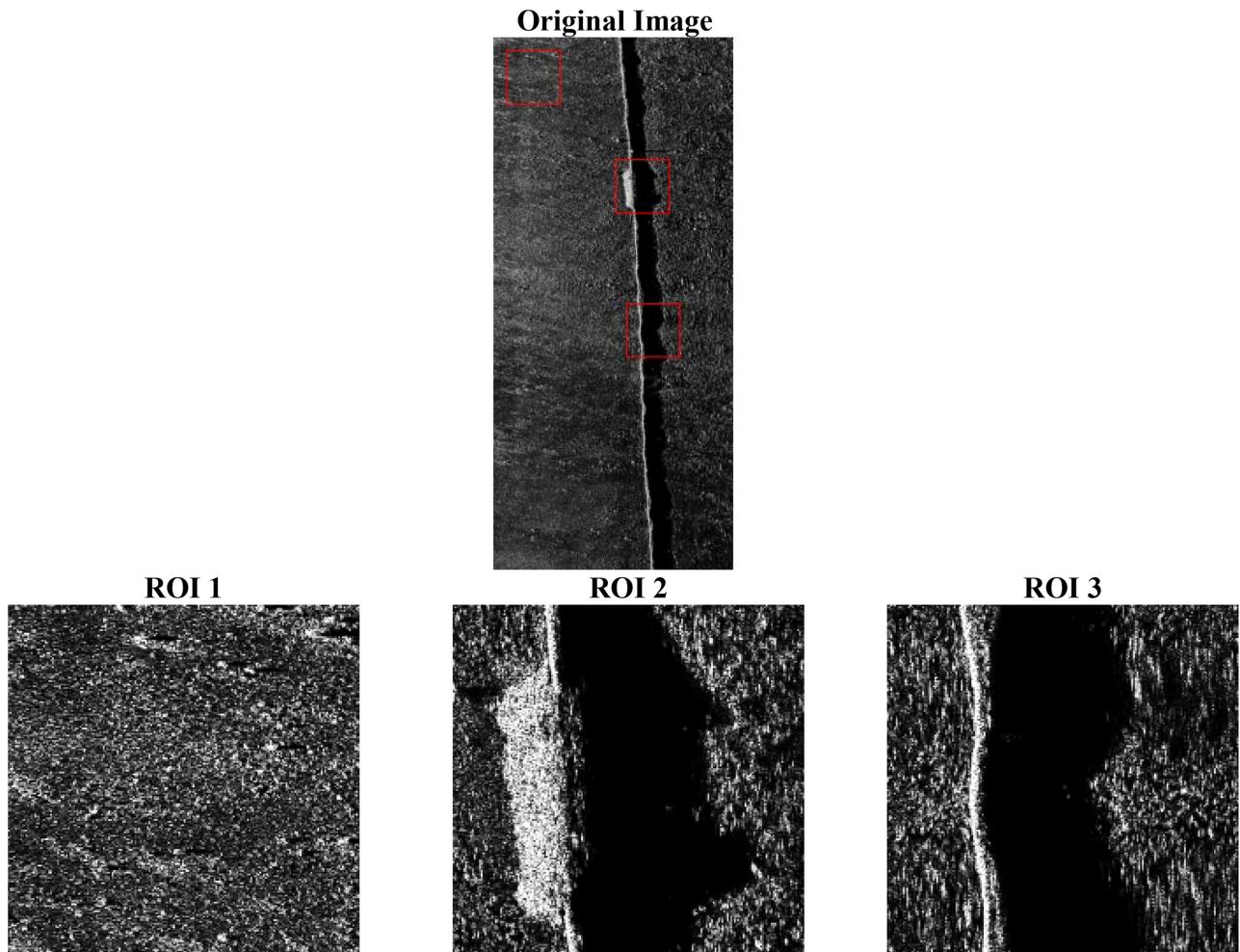
Fig. 8 Three ROI selected from sonar image with a pipeline on seafloor
