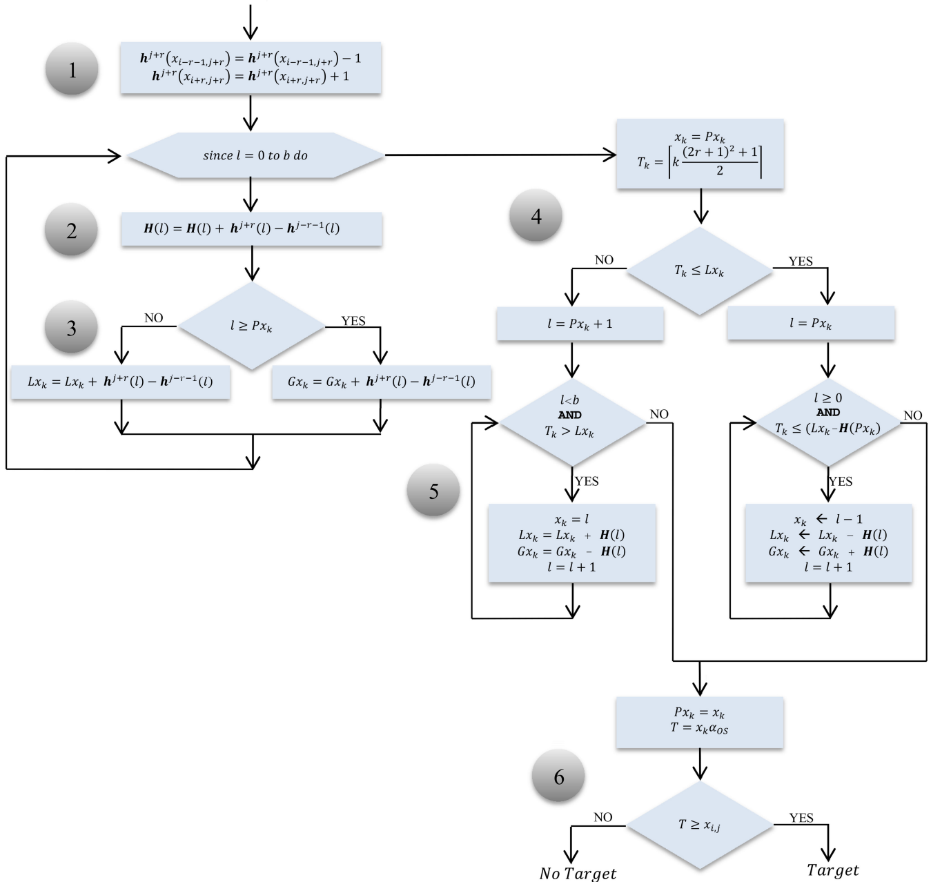
Fig. 4 Flowchart of the OS-CFAR 2D approach using distributive histograms and breakdown point optimal concept
