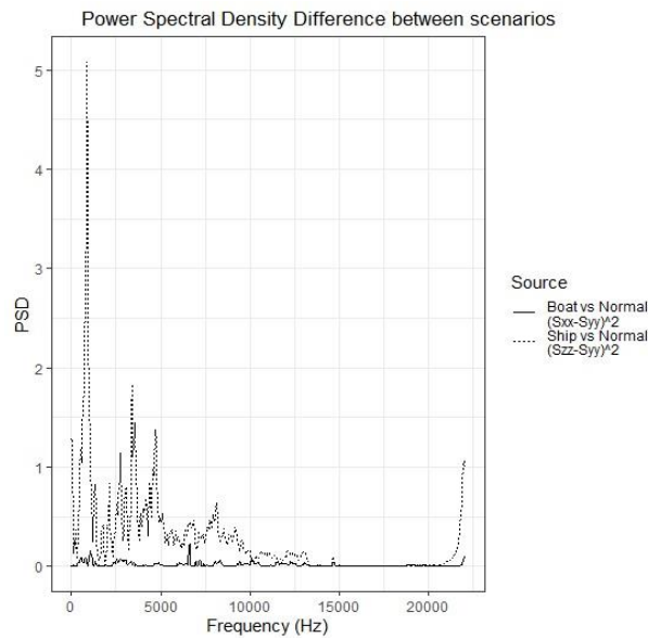
Fig.4 Power spectral density differences between two scenarios presented by the two types of vessels
