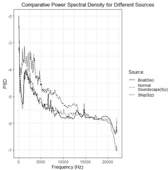
Fig.3 Comparison of the power spectral density of the normal soundscape (Syy)and the additional sources of sound, “boat” (Sxx) and “ship” (Szz)
