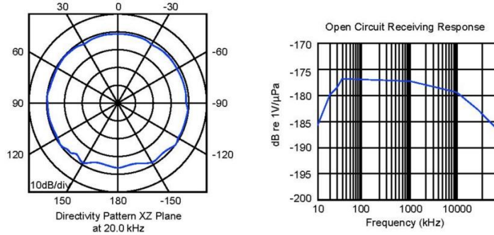
Fig. 1. Hydrophone directional responses and frequency response..
