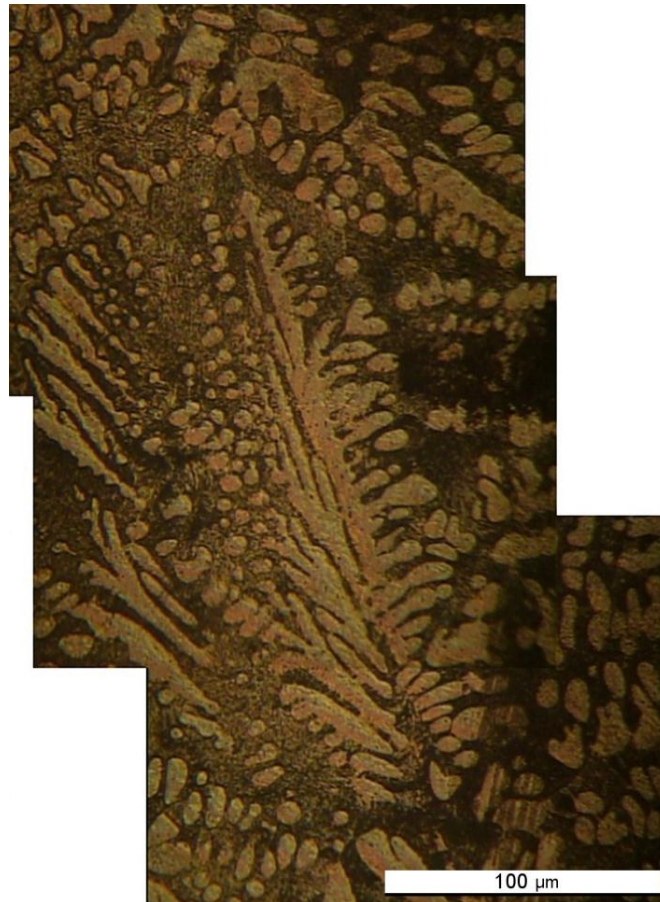
Fig. 4: Directional growth of \text{Sn-3.5\%Ag-0.9\%Cu} under V = 2 \mu\text{m/s} and G_L = 2.5 \text{ K/mm} .
