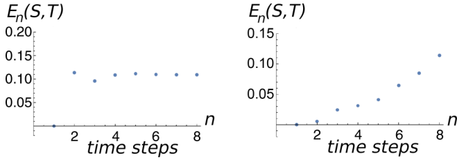
FIG. 6. System-time entanglement entropy E_n(S, T) vs number of steps, for the experimentally generated history states corresponding to the two eight-time-step trajectories of Table I.
