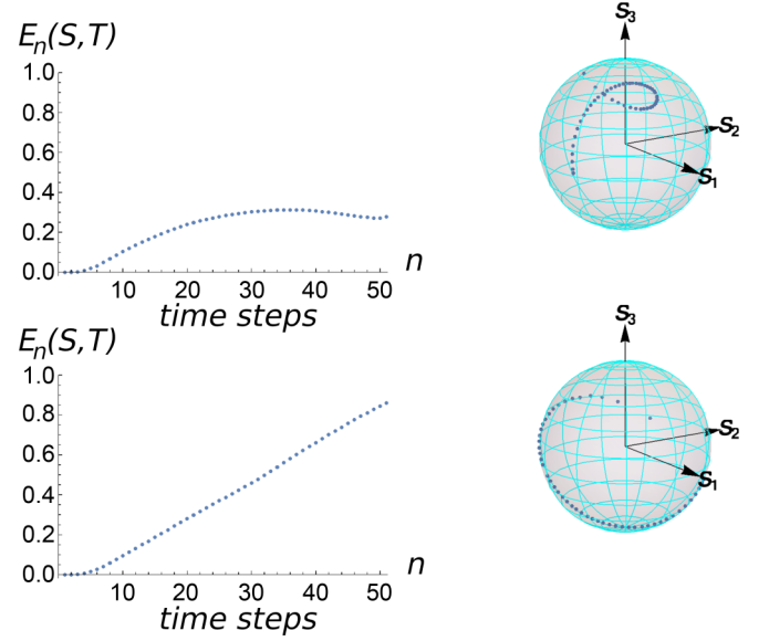
FIG. 5. System-time entanglement entropy E_n(S, T) vs number of steps (left panels) and trajectories in the polarization Bloch sphere (right panels) for two different initial states. The same set of 52 unitary evolution operators extracted from the experimental characterization was employed in both cases.
