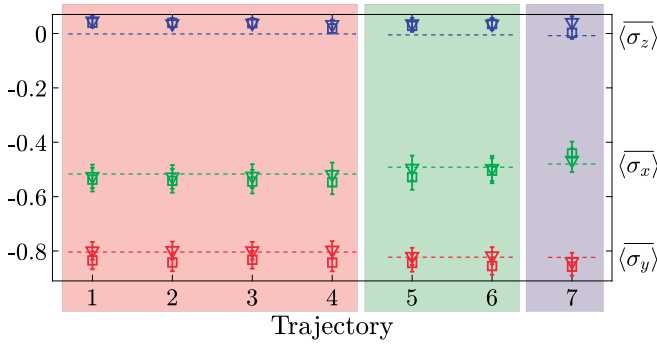
FIG. 4. Time averages of the polarization observables, \overline{\langle \sigma_\mu \rangle} , for different evolutions of the initial system state |\psi_0\rangle . The graphic shows the predicted values (---) in comparison with the experimental values, obtained by averaging over all spatial regions ( \square ), and by means of one single measurement ( \nabla ). Each sector, identified by a single color, indicates different evolutions through the same states |\psi_t\rangle .
