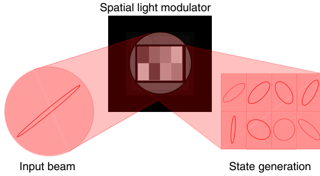
FIG. 1. Sketch of the action of the SLM on the initial state of light. The complex function \Gamma(\mathbf{x}) programmed on the SLM defines eight spatial regions in the region of interest, and each of them modifies the polarization state according to the particular gray level.
