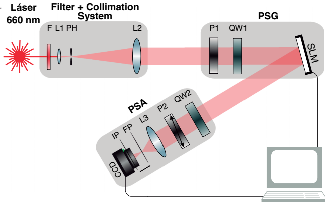
FIG. 2. Experimental setup used for the generation of history states and the subsequent characterization of the evolution of the quantum system S .
