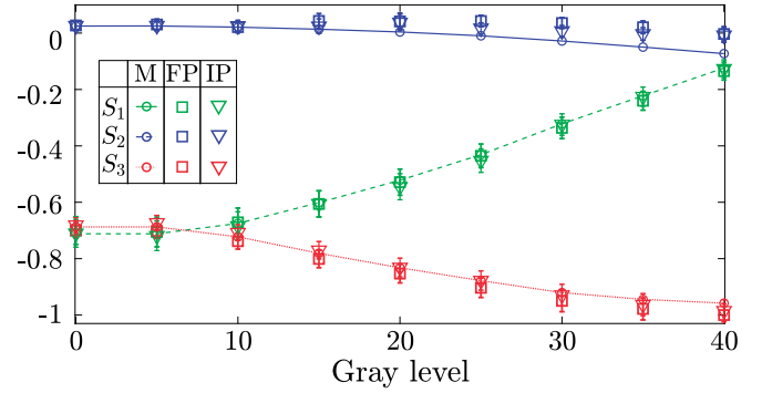
FIG. 3. Normalized Stokes parameters of the polarization state reflected by the SLM as a function of the gray level. The incoming polarization state is given by (S_0, S_1, S_2, S_3) = (1.000, 0.040, 0.951, -0.026) . The graphic shows the experimental values obtained by a measurement in the IP ( \nabla ) or in the FP ( \square ), in comparison with those predicted by the Mueller matrix ( \circ ).
