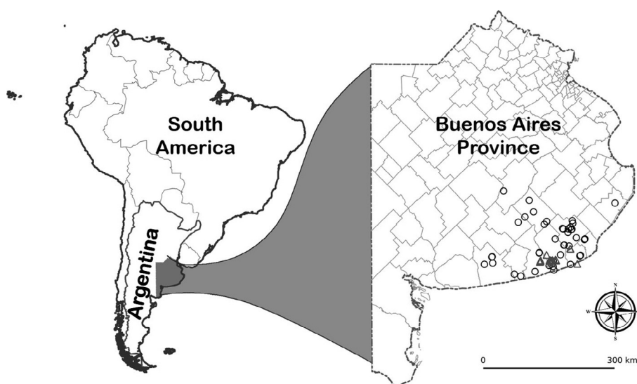
Fig. 1. Sampling sites throughout the southeastern Buenos Aires province at the Argentinean Pampas. ○: sampling sites to evaluate relationships among variables and regression model fitting ( n = 46 ), △: sampling sites for model validation ( n = 32 ). Only the location of continuous cropping (CC) plots is shown because the location of pseudo-pristine plots was very close to the CC plots (no more than 500 m away).
