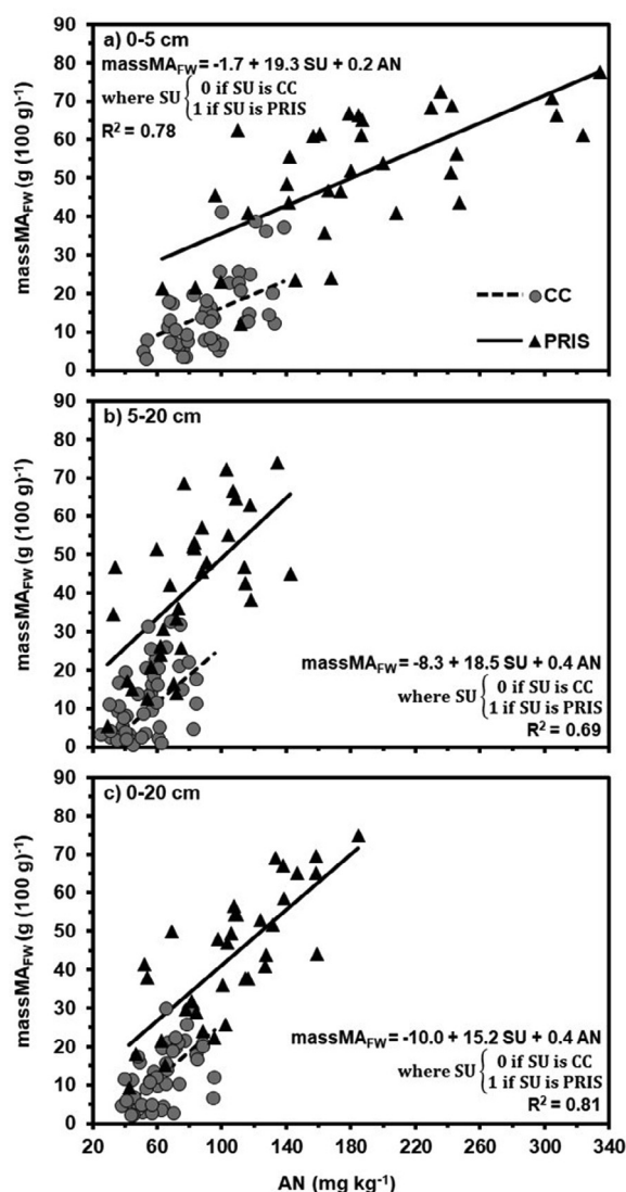
Fig. 5. Relationship between 2000 and 8000 \mu\text{m} macroaggregate mass after fast wetting ( \text{massMA}_{\text{FW}} ) and anaerobically mineralizable nitrogen (AN) for two soil uses at three depths: 0–5 (a), 5–20 (b), and 0–20 cm (c). n = 80 . P < 0.05 . SU: soil use. CC: continuous cropping ( n = 46 ). PRIS: pseudo-pristine ( n = 34 ).
