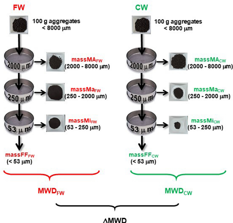
Fig. 2. Scheme of aggregate separation methodology. FW: fast wetting, CW: capillary wetting, MWD: mean weight diameter, ΔMWD: difference of MWD between CW and FW, massMA: 2000–8000 μm macroaggregate mass, massMa: 250–2000 μm macroaggregate mass, massMi: microaggregate mass, massFF: fine fraction mass.
