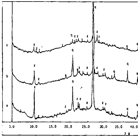
Figure 1 Diffractograms of the reaction products. a) Concrete N 1, b) Concrete N 2, c) Concrete N 3
