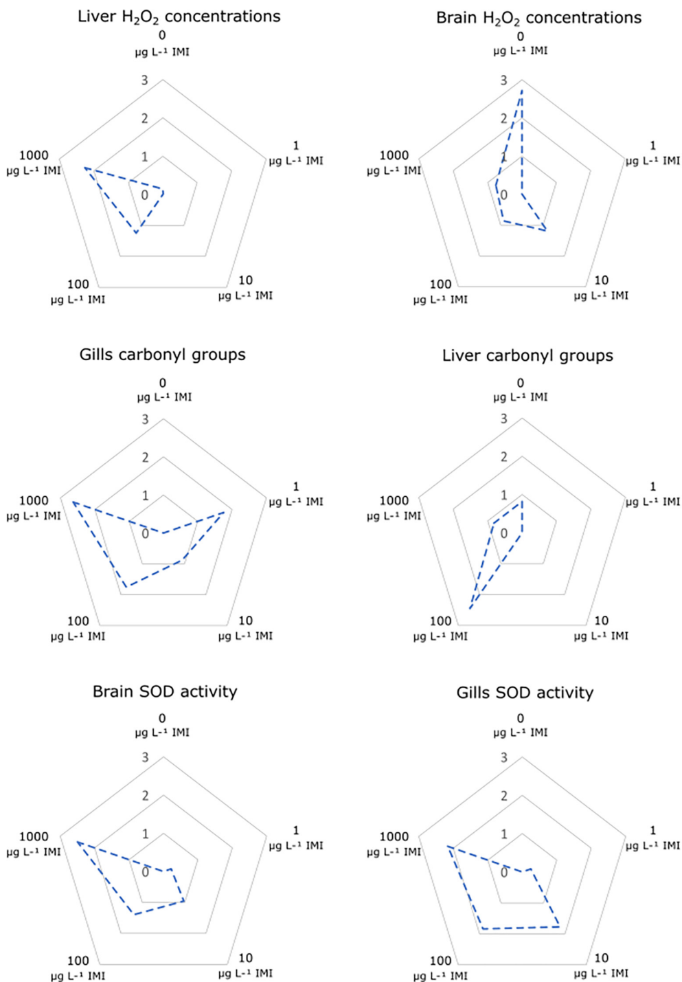
Fig. 2. Weight (standardized value, S) of considered biomarkers used to calculate the Integrated Biomarker Response (IBR) index for Australoheros facetus exposed during 48 h to different treatments: 0 (Control), 1, 10, 100 and 1000 \mu\text{g L}^{-1} of imidacloprid (IMI). The spokes of the radar indicate the S value for each treatment.
