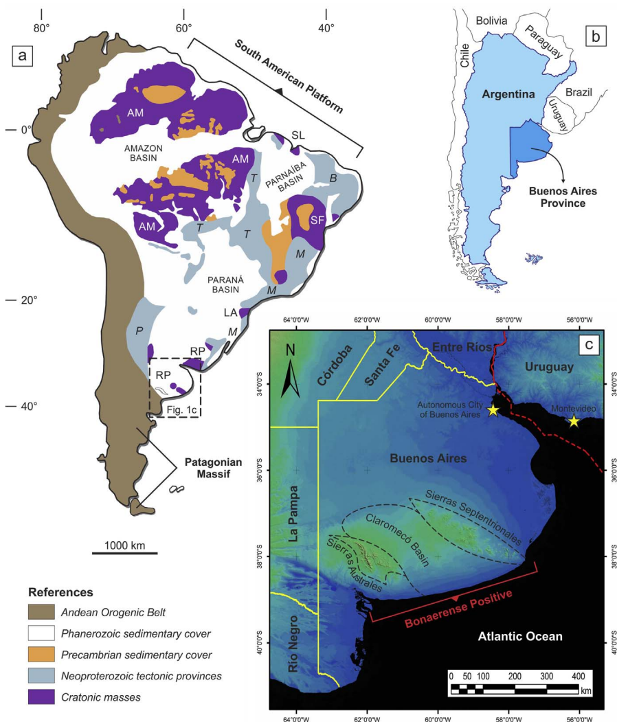
Fig. 1. a) Geological map of South America with emphasis on the South American Platform (modified from Basei et al. (2010)). b) Political map of Argentina, indicating the Buenos Aires Province. c) LANDSAT satellite image of the Buenos Aires Province, indicating the morphostructural units that make up the Bonaerense Positive. Cratons: AM = Amazonian, SL = São Luís, SF = São Francisco, LA = Luiz Alves, RP = Río de la Plata. Neoproterozoic tectonic provinces: B = Borborema, T = Tocantins, M = Mantiqueira, P = Pampean.
