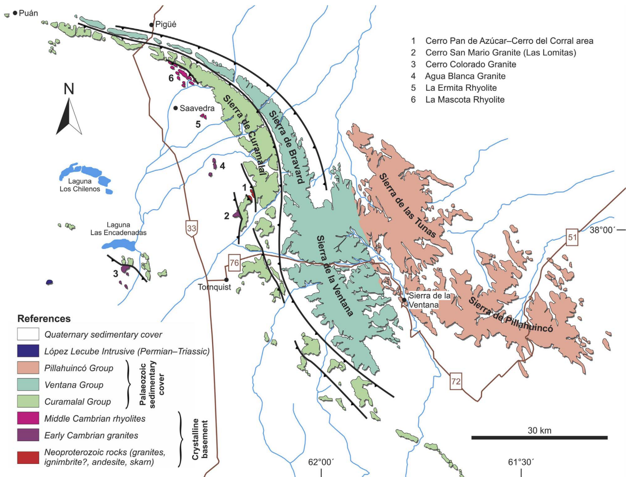
Fig. 2. Geological map of the Ventania System (modified from Ramos et al. (2014)).
