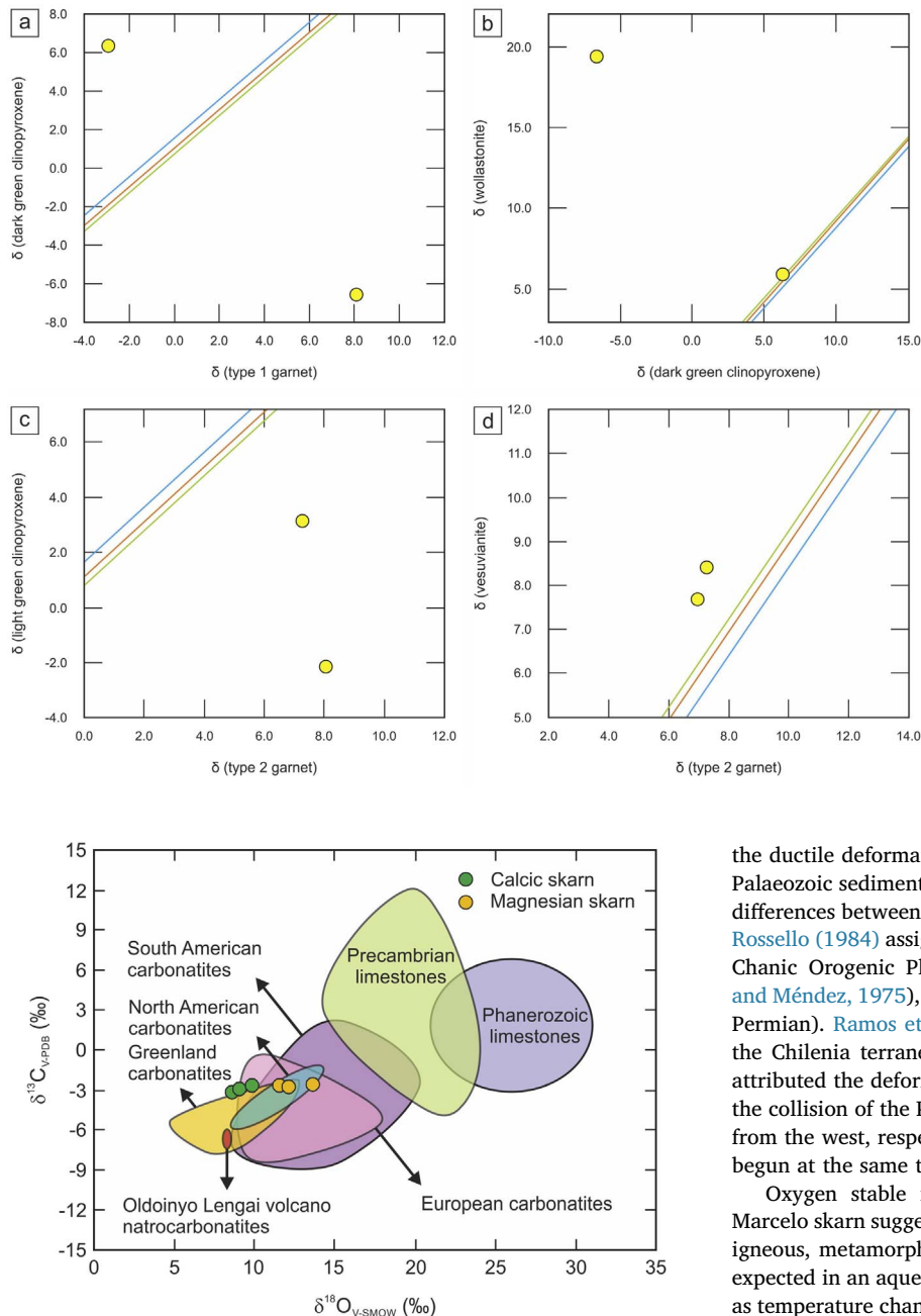
Fig. 20. Comparison of the stable isotope compositions between the Loma Marcelo skarn, limestones of different ages, and carbonatites from different continents (isotope data from Ballivián Justiniano et al. (2015), modified from Bell and Simonetti (2009)).
