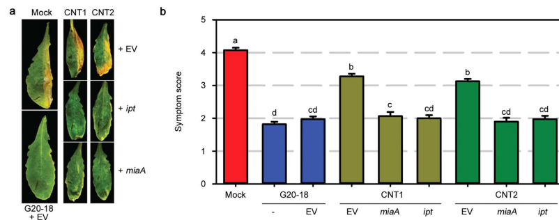
Figure 2. Complementation of the CNT transposon mutants with a functional CK biosynthetic gene restores their biocontrol ability. (a) The biocontrol ability of CNT transposon mutants is restored by complementation with functional Atipt or G20-18 miaA evident from strongly reduced Pto symptoms (right leaf halves) 4 days post infection (dpi) with 10^6 cfu ml ^{-1} . Transformation with the empty vector pBBRMCS-5 (EV) has no effect. (b) Average Pto symptom score in Arabidopsis 4 dpi with 10^6 cfu ml ^{-1} after indicated pre-treatments. Data are means \pm s.e. n \geq 226 , letters indicate different significance groups ( P < 0.05 ).
