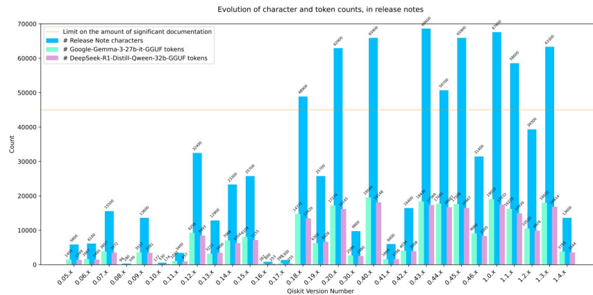
Fig. 4. Qiskit release notes size distribution
