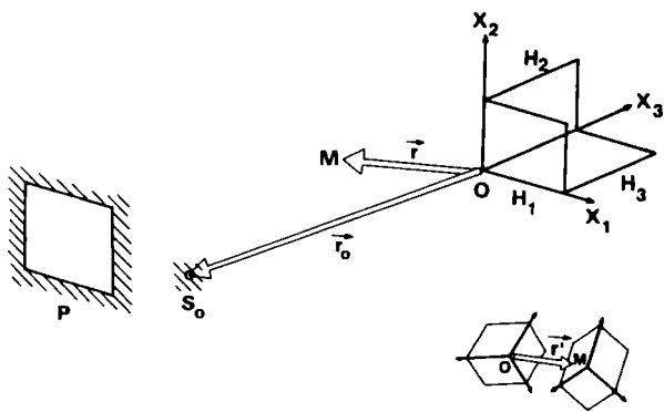
Fig. 1. Scheme of the experimental setup: H_1 , H_2 , and H_3 are three recording plates in a trihedral arrangement, \mathbf{r} denotes a point position vector on one of the plates, \mathbf{r}' indicates the position vector of the same point after the trihedral motion, and \mathbf{r}_0 is the position vector of the reference source S_0 . P is an empty pupil which diffracts an approximately plane wave.
